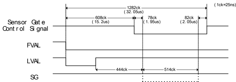
Fig. 29A. Sensor Gate Control single channel details
